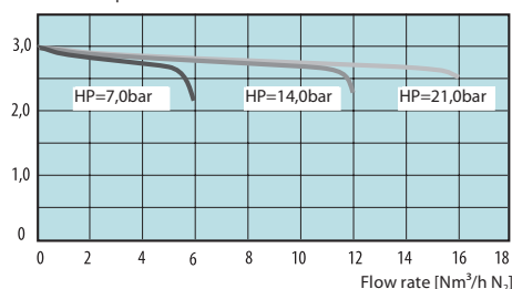
Down stream pressure
